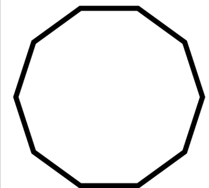
Decagon
