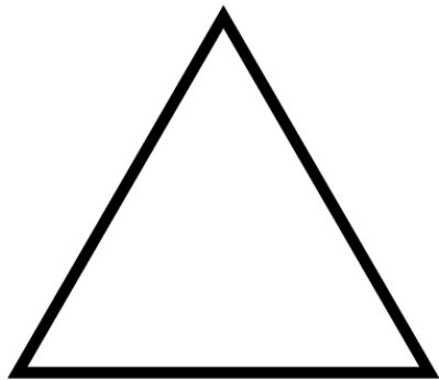
Triangle
