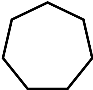
Heptagon
