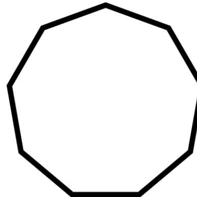
Nonagon
